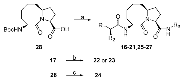
Scheme 1. General Synthesis of Conformationally Constrained [8,5] Bicyclic Smac Mimetics a
